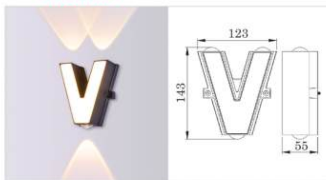
CHỮ V LED 10W - 3000K 780.000đ
