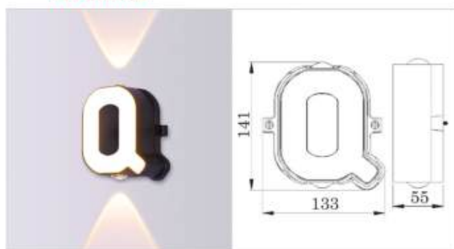
CHỮ Q LED 10W - 3000K 780.000đ
