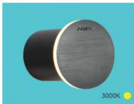
ACT-50 LED 3W - 220V Ø65 x H70 - Ip54 900.000đ
