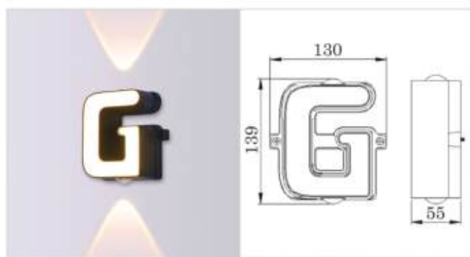
CHỮ G LED 10W - 3000K 780.000đ
